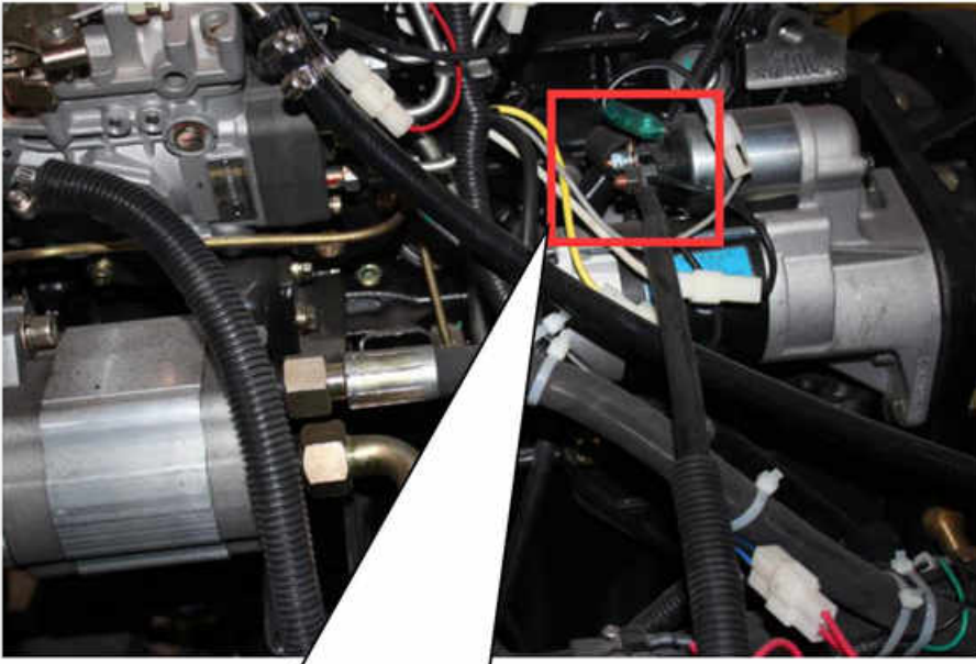
12V Positive Pole connect with JMC auxiliary engine Negative Pole connect with chassis
